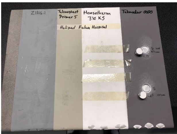
The coating system for the supporting beams & cross bracings on the 4 parking levels under the FALUN Hospital Helipad.
